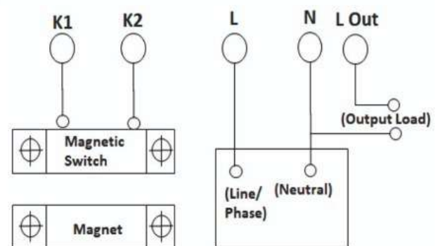
1L-AC101S - SINGLE DOOR CONNECTION
